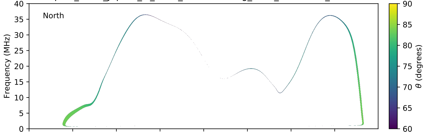
expres_earth_jupiter_io_isaac_lossc-wid1deg_3kev_20151110_v01.cdf
