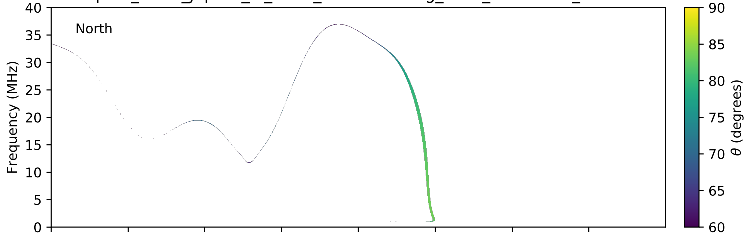
expres_earth_jupiter_io_isaac_lossc-wid1deg_3kev_20151105_v01.cdf
