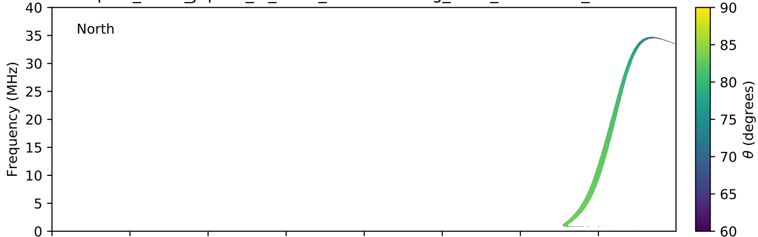
expres_earth_jupiter_io_isaac_lossc-wid1deg_3kev_20151104_v01.cdf
