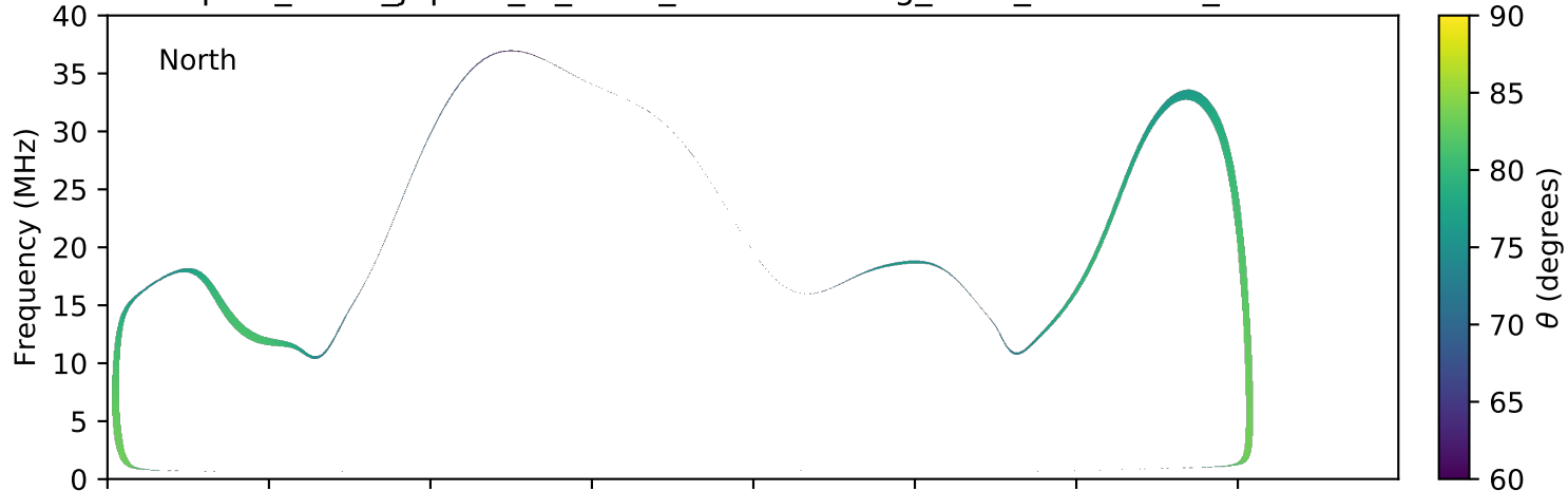
expres_earth_jupiter_io_isaac_lossc-wid1deg_3kev_20151103_v01.cdf
