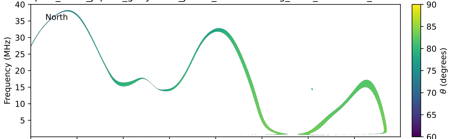
expres_earth_jupiter_ganymede_jrm33_lossc-wid1deg_3kev_20151117_v11.cdf
