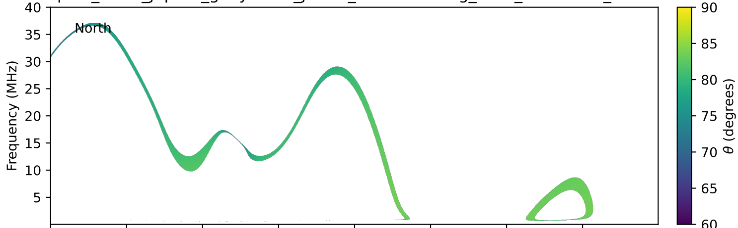
expres_earth_jupiter_ganymede_jrm33_lossc-wid1deg_3kev_20151110_v11.cdf
