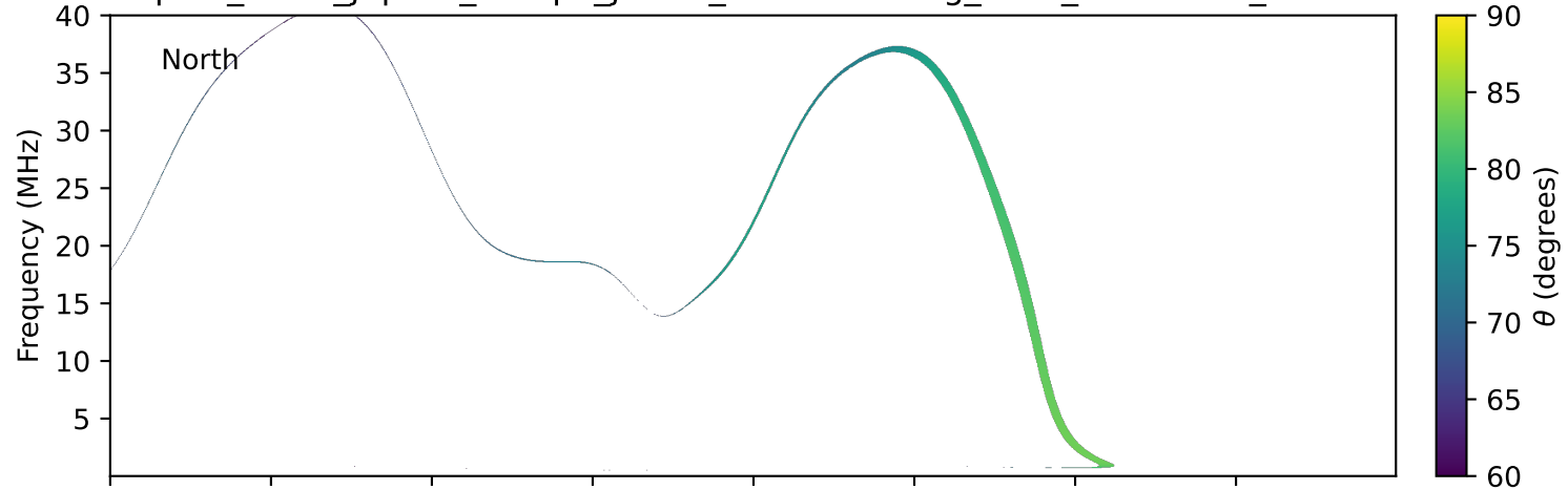
expres_earth_jupiter_europa_jrm33_lossc-wid1deg_3kev_20151126_v11.cdf
