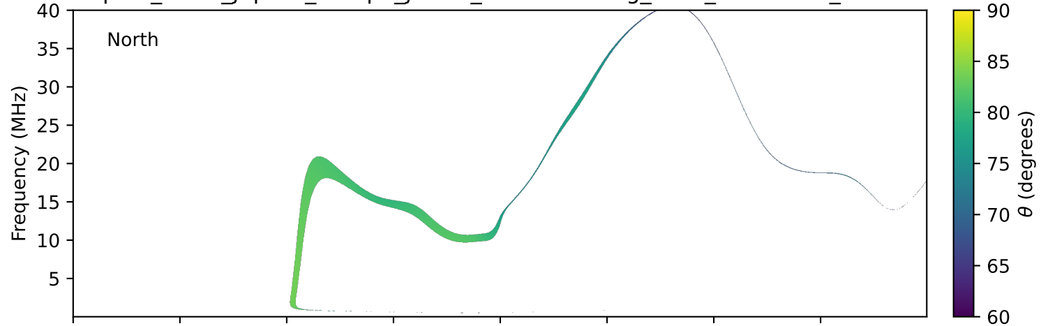
expres_earth_jupiter_europa_jrm33_lossc-wid1deg_3kev_20151125_v11.cdf
