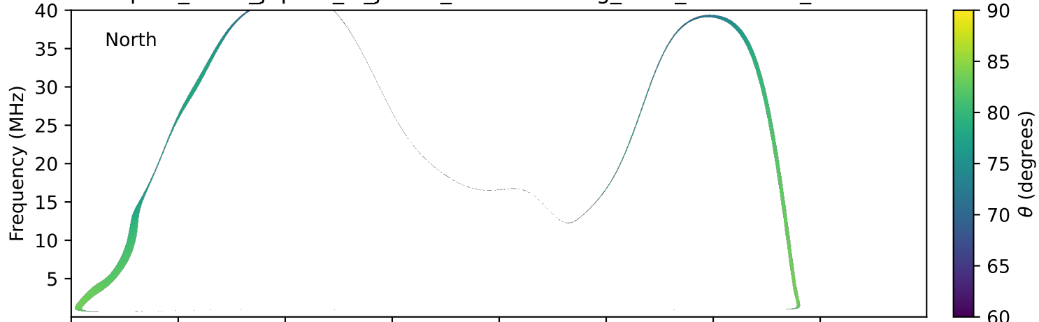
expres_earth_jupiter_io_jrm33_lossc-wid1deg_3kev_20151025_v11.cdf
