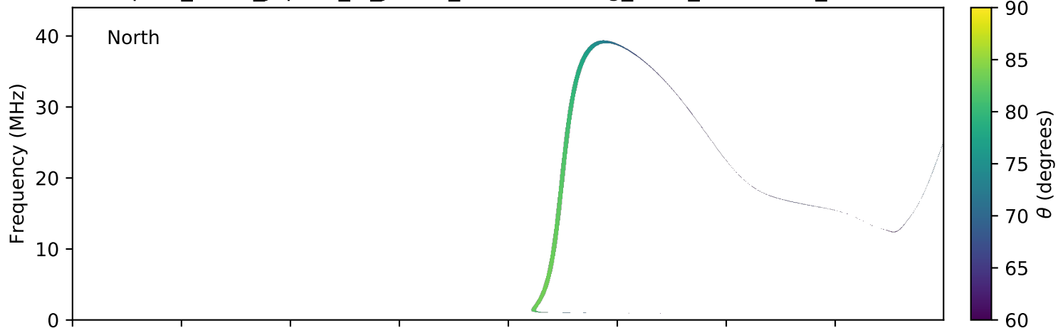
expres_earth_jupiter_io_jrm09_lossc-wid1deg_3kev_20151030_v01.cdf
