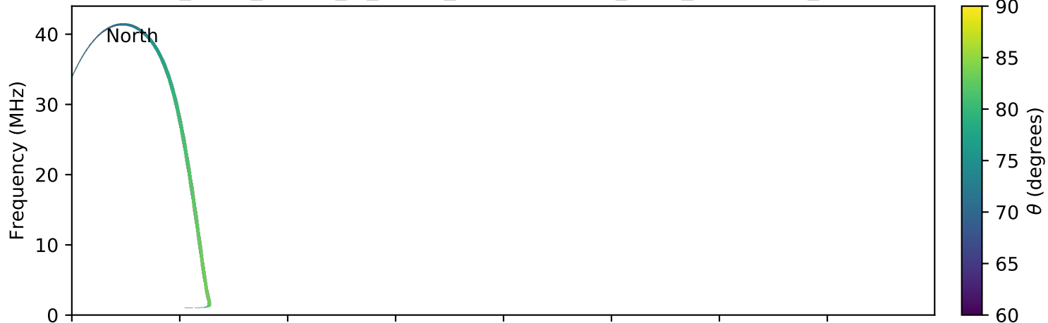
expres_earth_jupiter_io_jrm09_lossc-wid1deg_3kev_20151017_v01.cdf
