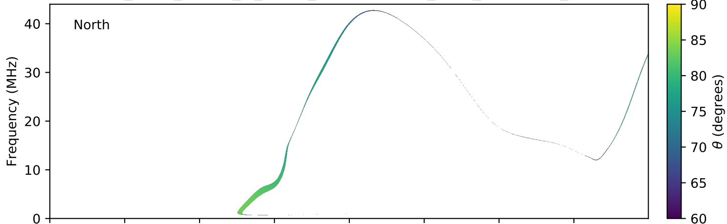
expres_earth_jupiter_io_jrm09_lossc-wid1deg_3kev_20151016_v01.cdf
