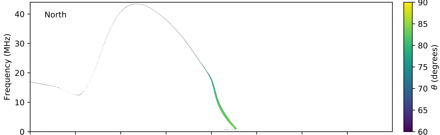
expres_earth_jupiter_io_jrm09_lossc-wid1deg_3kev_20151013_v01.cdf
