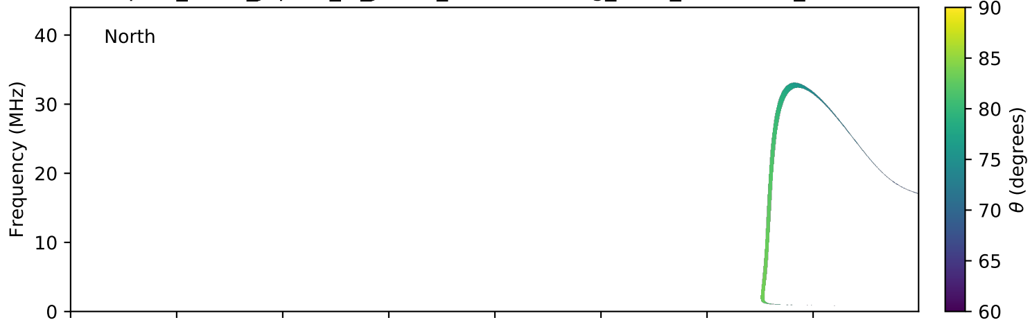
expres_earth_jupiter_io_jrm09_lossc-wid1deg_3kev_20151012_v01.cdf
