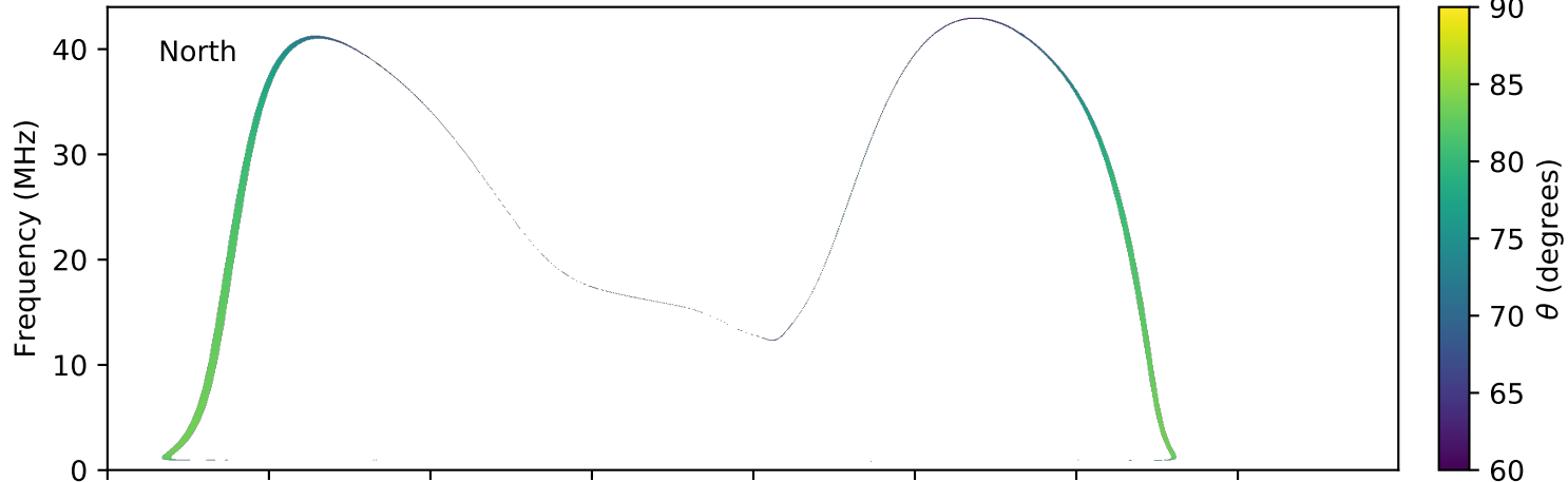
expres_earth_jupiter_io_jrm09_lossc-wid1deg_3kev_20151011_v01.cdf
