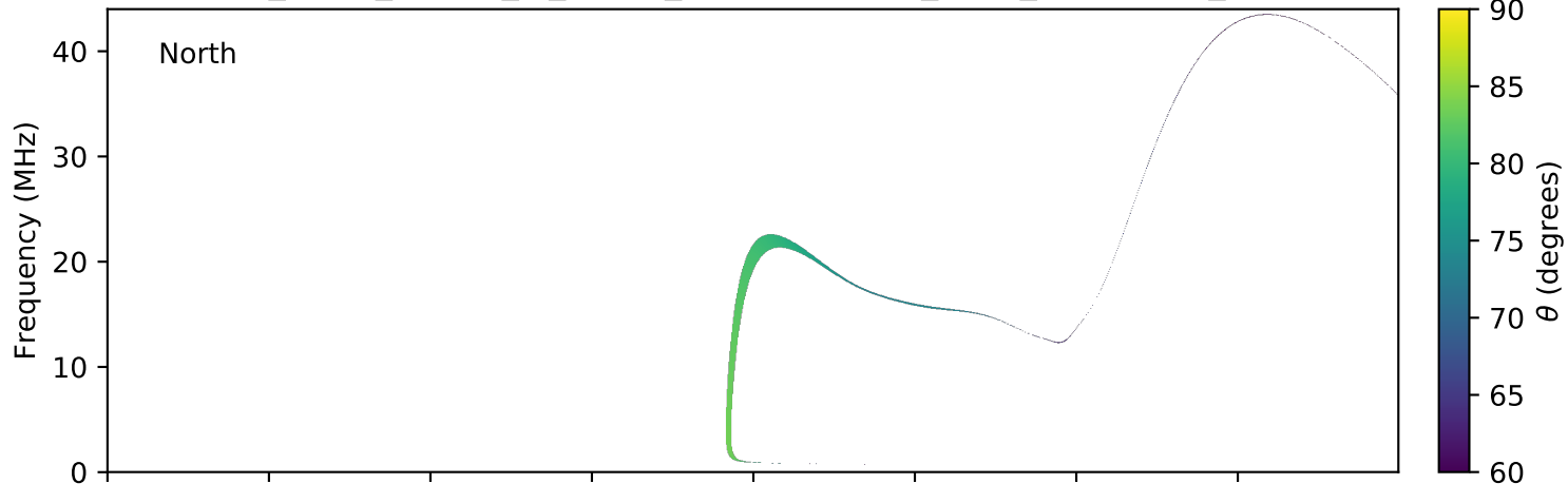
expres_earth_jupiter_io_jrm09_lossc-wid1deg_3kev_20151007_v01.cdf
