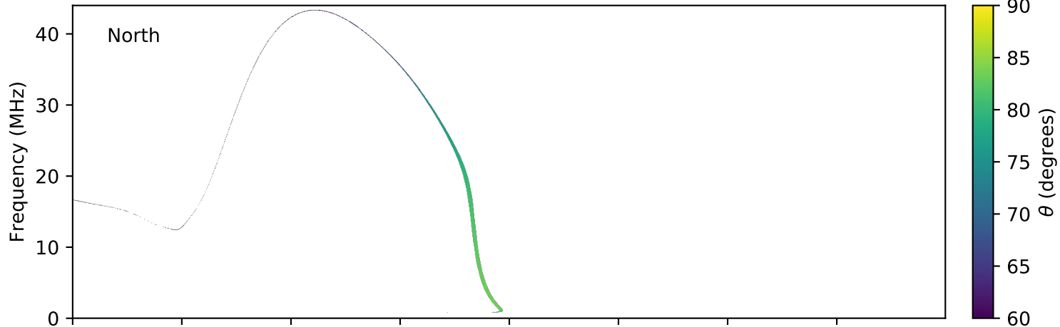
expres_earth_jupiter_io_jrm09_lossc-wid1deg_3kev_20151006_v01.cdf
