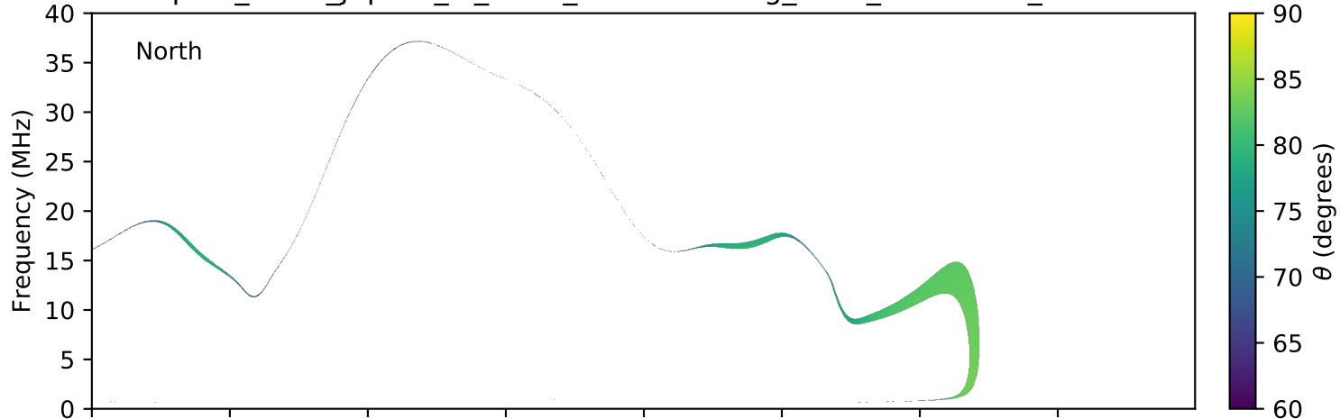
expres_earth_jupiter_io_isaac_lossc-wid1deg_3kev_20151027_v01.cdf
