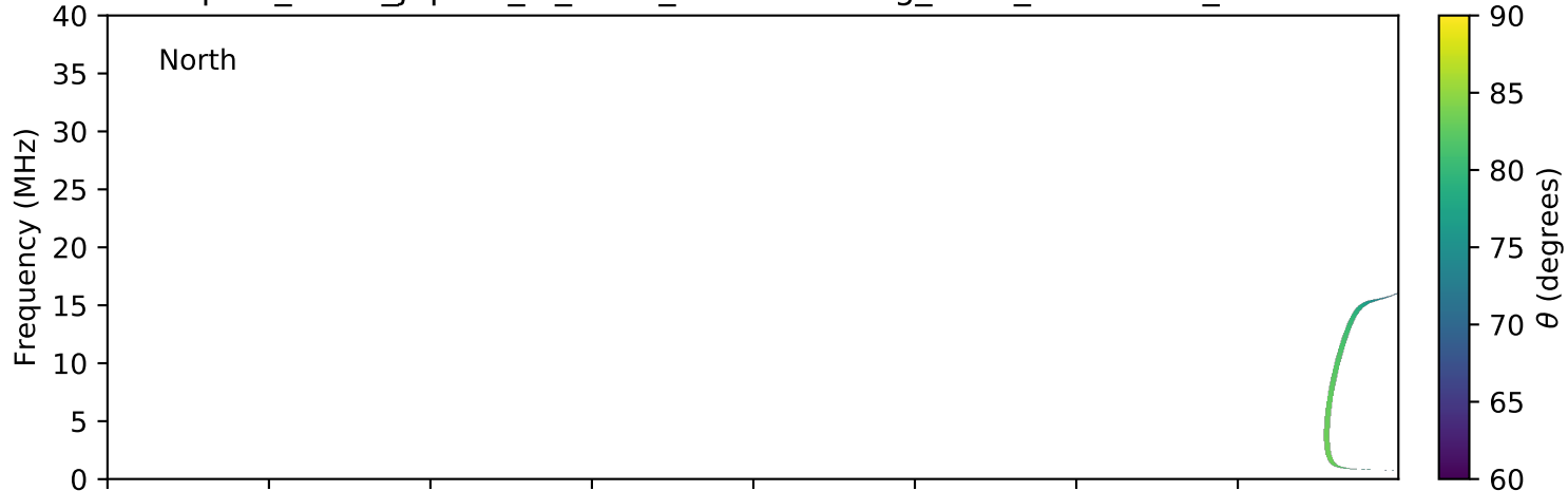
expres_earth_jupiter_io_isaac_lossc-wid1deg_3kev_20151026_v01.cdf
