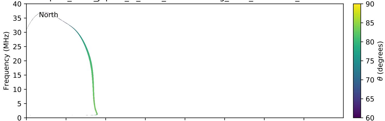
expres_earth_jupiter_io_isaac_lossc-wid1deg_3kev_20151024_v01.cdf
