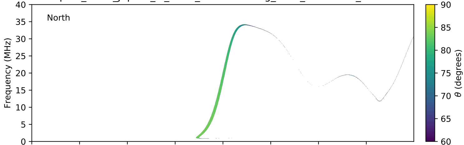
expres_earth_jupiter_io_isaac_lossc-wid1deg_3kev_20151023_v01.cdf
