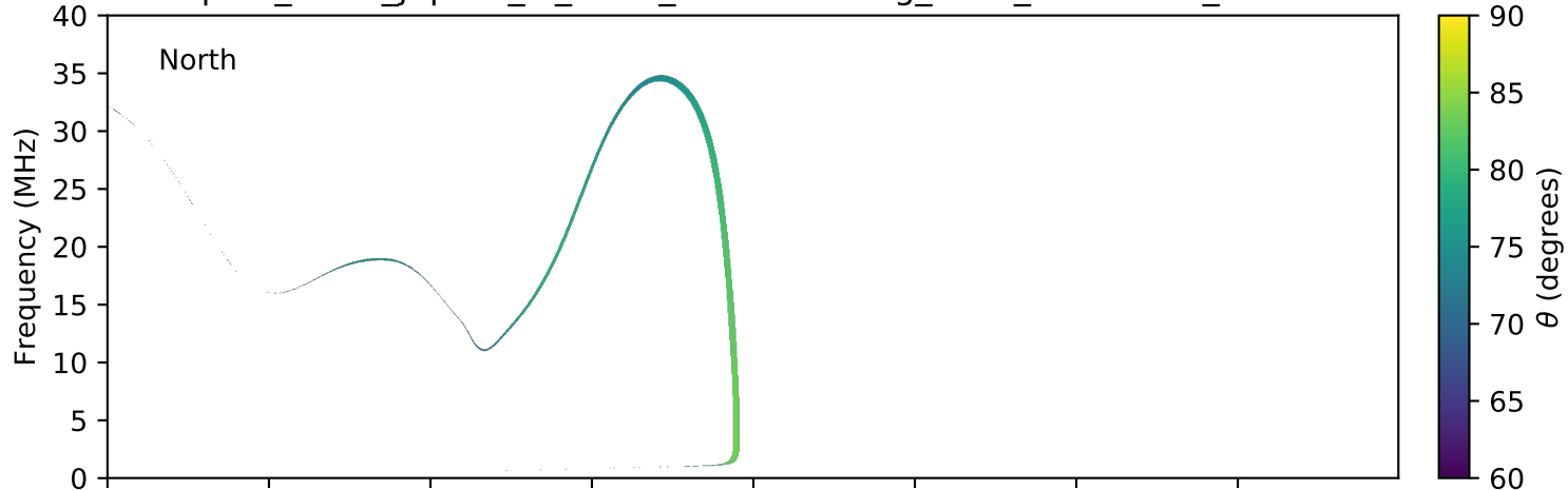
expres_earth_jupiter_io_isaac_lossc-wid1deg_3kev_20151022_v01.cdf
