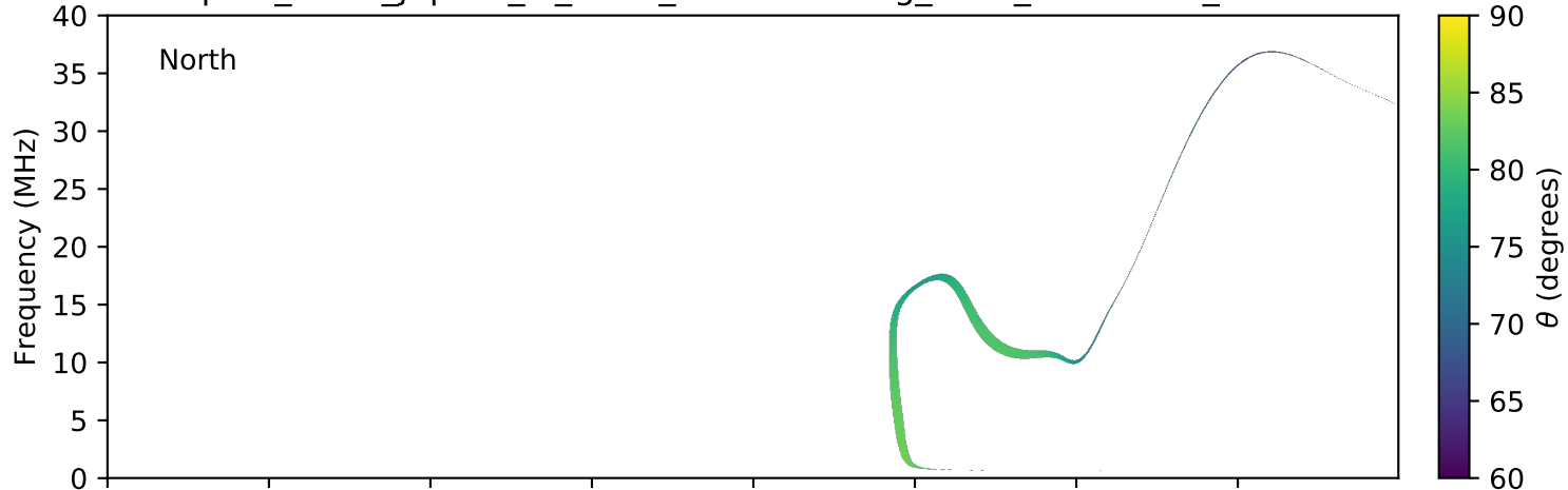
expres_earth_jupiter_io_isaac_lossc-wid1deg_3kev_20151021_v01.cdf
