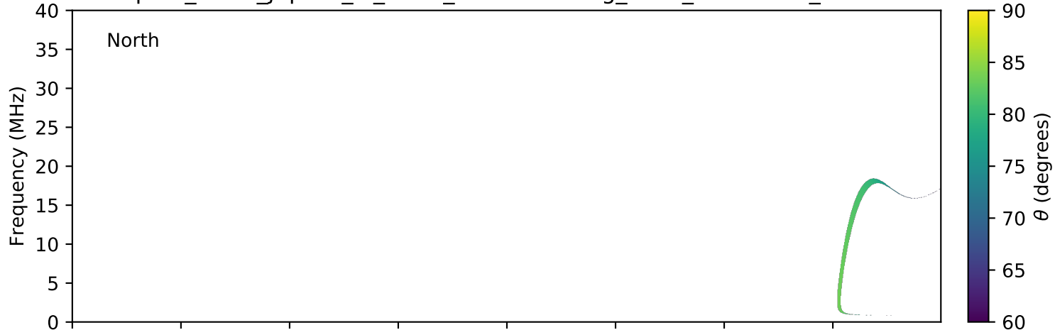
expres_earth_jupiter_io_isaac_lossc-wid1deg_3kev_20151019_v01.cdf
