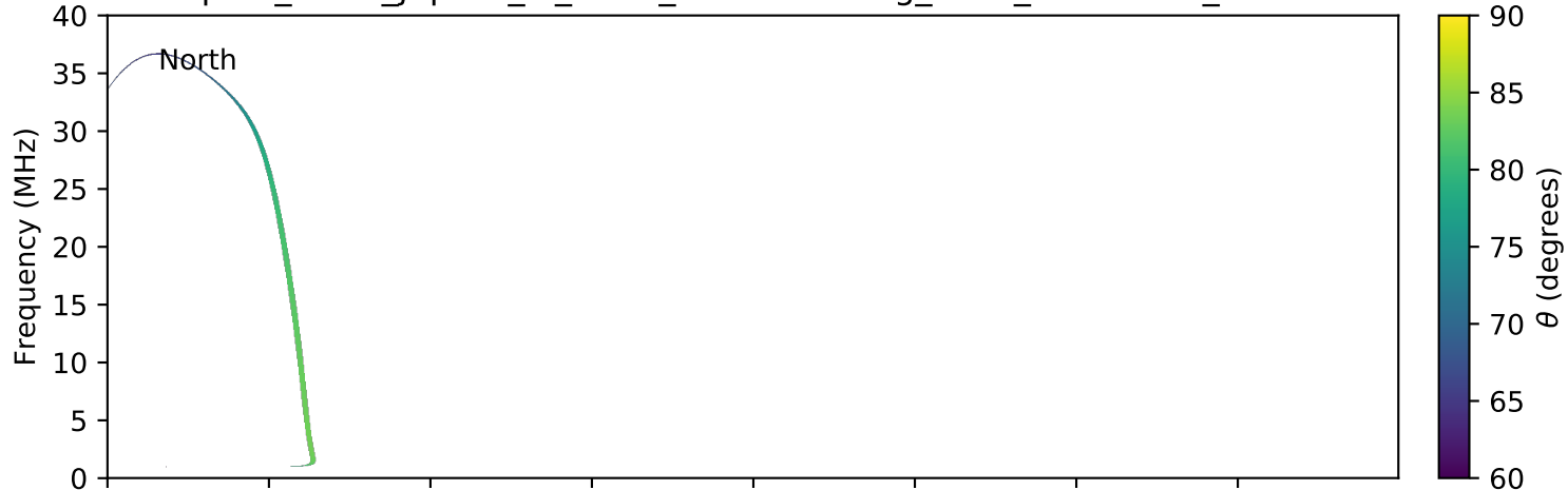
expres_earth_jupiter_io_isaac_lossc-wid1deg_3kev_20151017_v01.cdf
