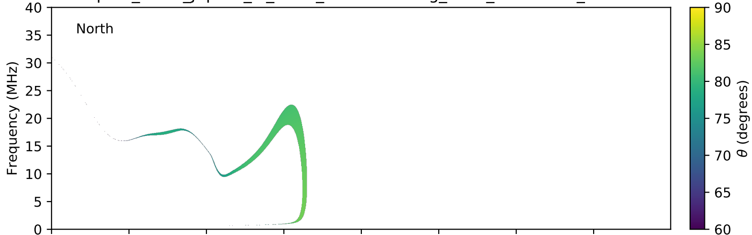
expres_earth_jupiter_io_isaac_lossc-wid1deg_3kev_20151015_v01.cdf
