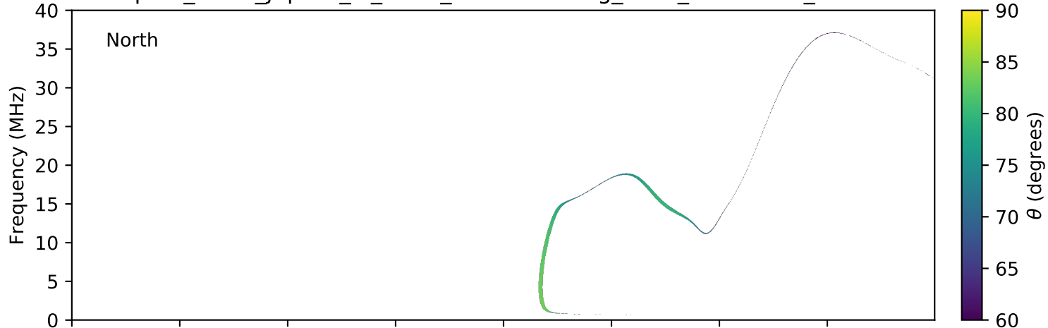
expres_earth_jupiter_io_isaac_lossc-wid1deg_3kev_20151014_v01.cdf
