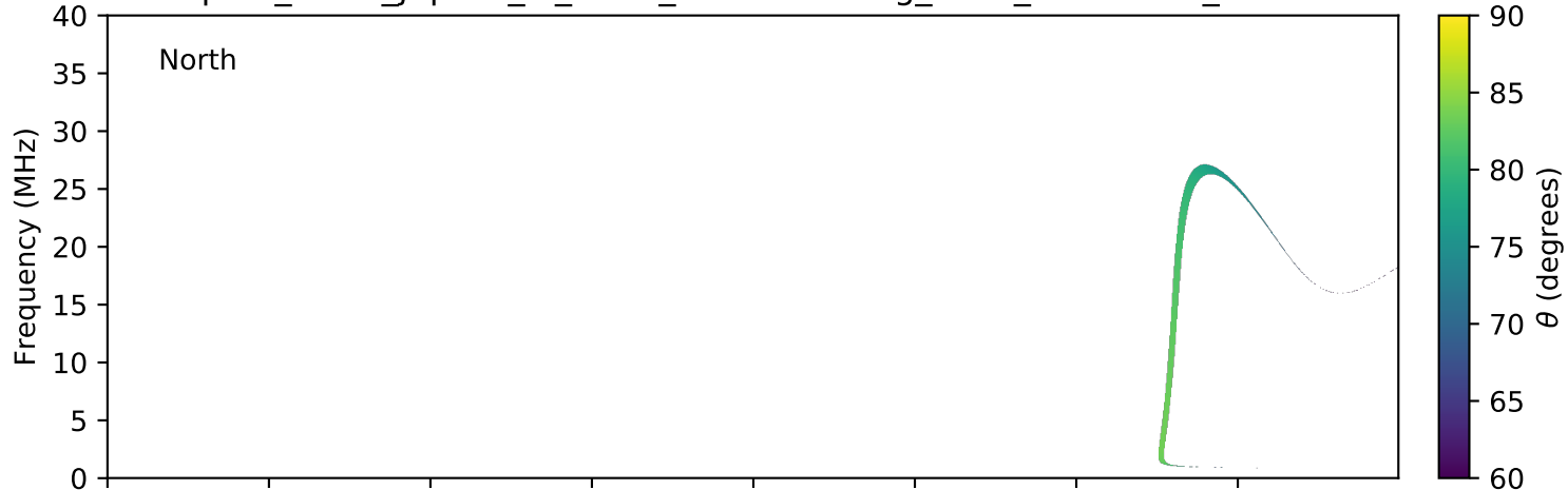
expres_earth_jupiter_io_isaac_lossc-wid1deg_3kev_20151012_v01.cdf
