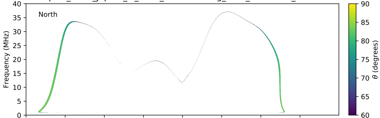
expres_earth_jupiter_io_isaac_lossc-wid1deg_3kev_20151011_v01.cdf
