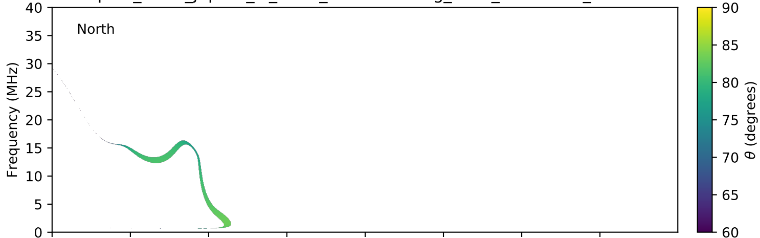
expres_earth_jupiter_io_isaac_lossc-wid1deg_3kev_20151008_v01.cdf
