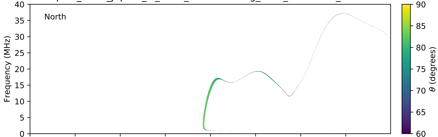
expres_earth_jupiter_io_isaac_lossc-wid1deg_3kev_20151007_v01.cdf
