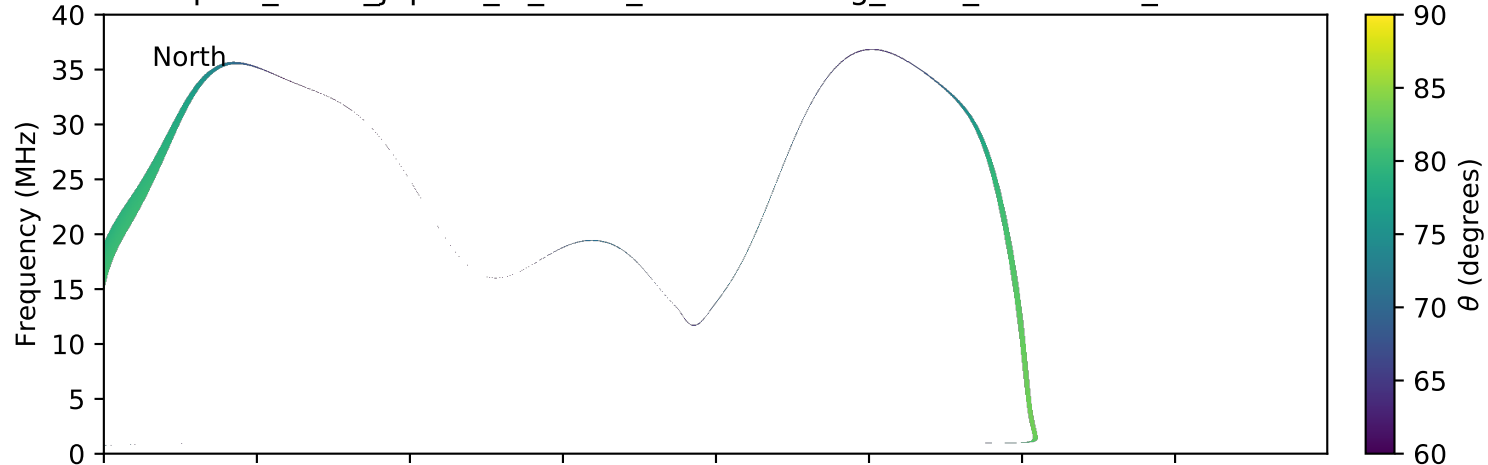
expres_earth_jupiter_io_isaac_lossc-wid1deg_3kev_20151004_v01.cdf
