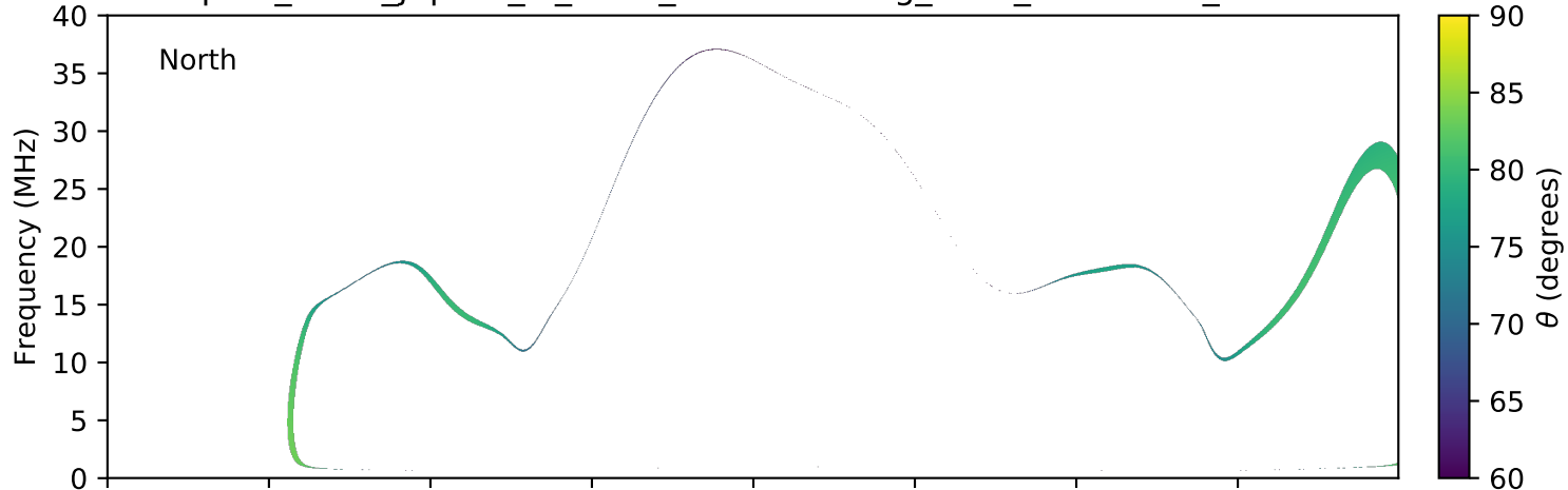
expres_earth_jupiter_io_isaac_lossc-wid1deg_3kev_20151002_v01.cdf
