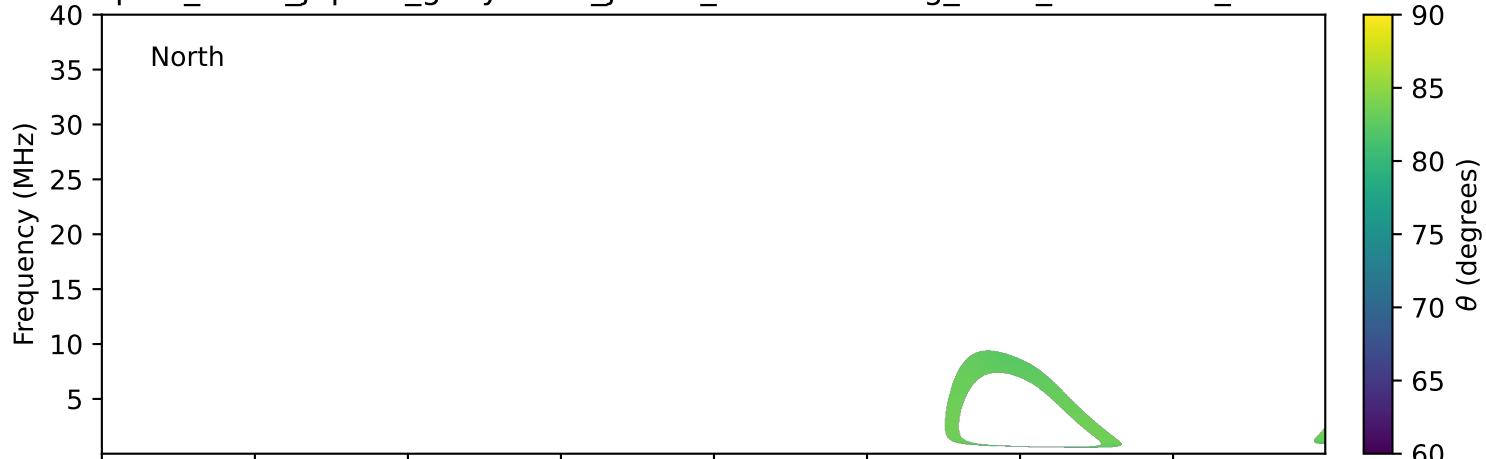
expres_earth_jupiter_ganymede_jrm33_lossc-wid1deg_3kev_20151013_v11.cdf
