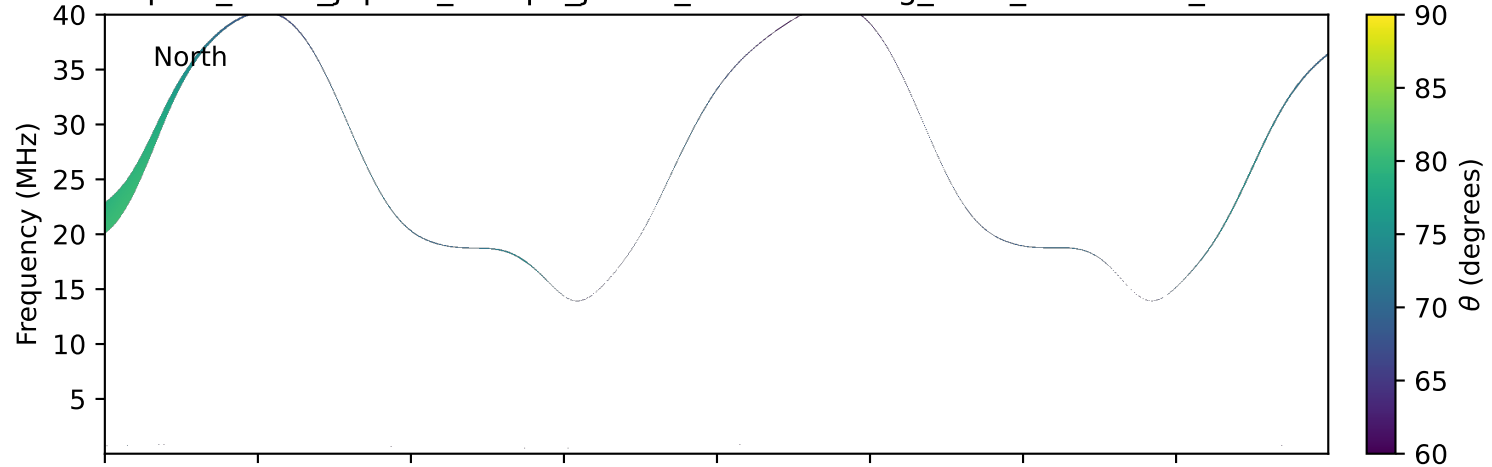
expres_earth_jupiter_europa_jrm33_lossc-wid1deg_3kev_20151009_v11.cdf
