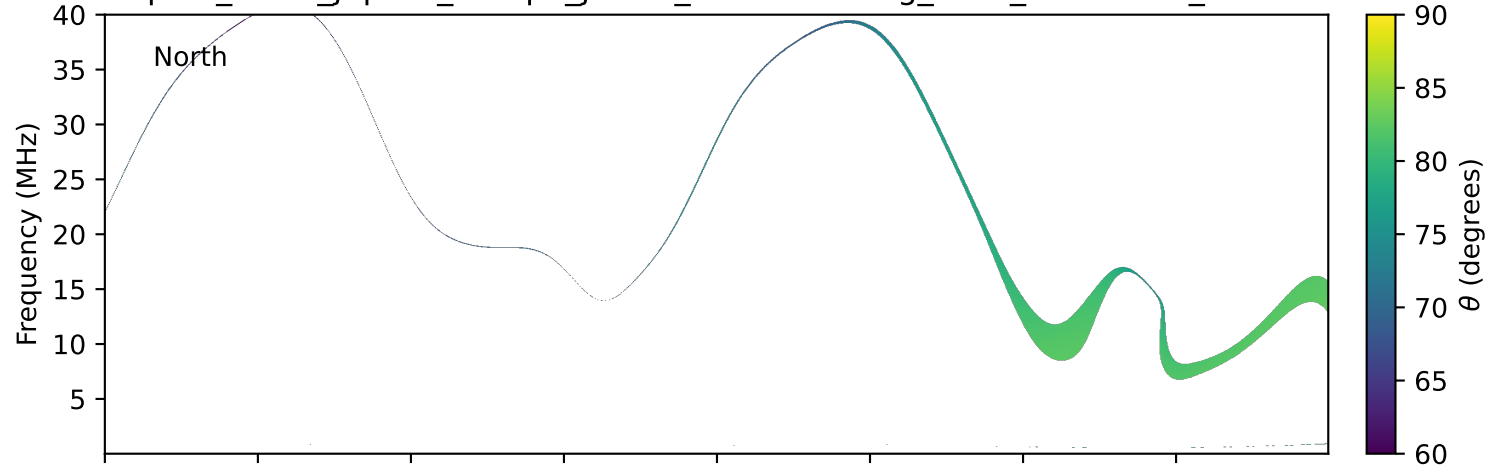
expres_earth_jupiter_europa_jrm33_lossc-wid1deg_3kev_20151002_v11.cdf
