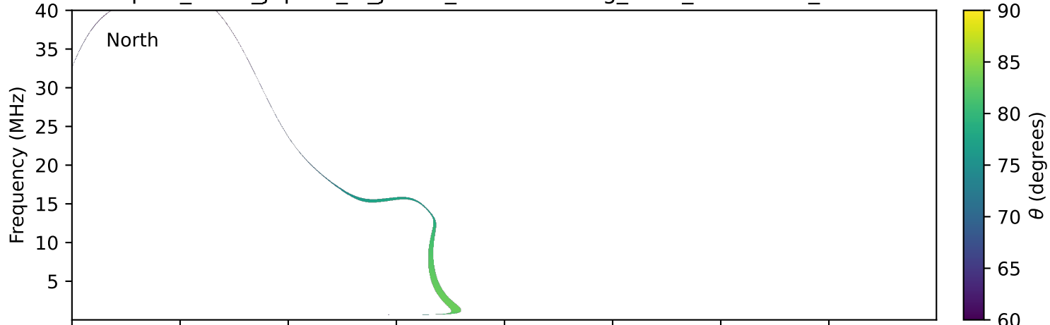
expres_earth_jupiter_io_jrm33_lossc-wid1deg_3kev_20150925_v11.cdf
