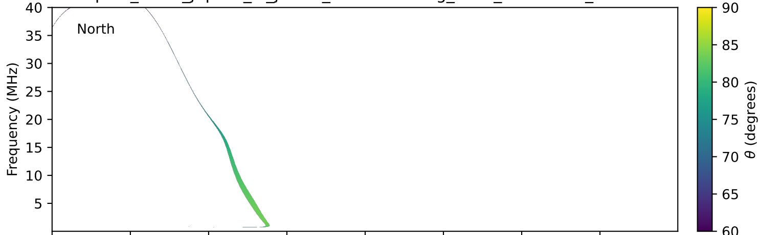
expres_earth_jupiter_io_jrm33_lossc-wid1deg_3kev_20150918_v11.cdf
