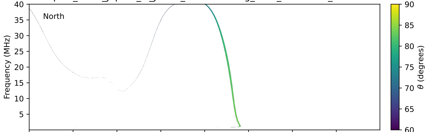
expres_earth_jupiter_io_jrm33_lossc-wid1deg_3kev_20150916_v11.cdf
