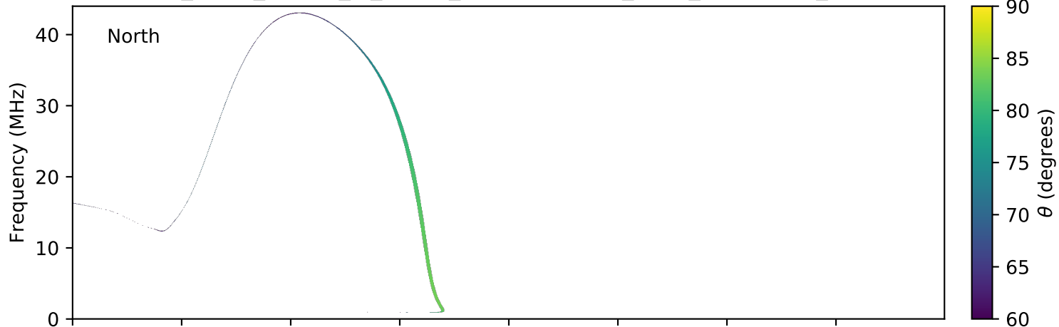
expres_earth_jupiter_io_jrm09_lossc-wid1deg_3kev_20150929_v01.cdf
