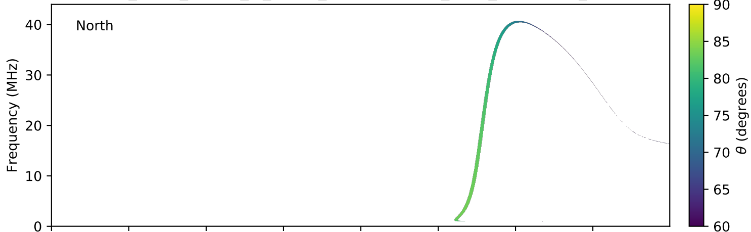
expres_earth_jupiter_io_jrm09_lossc-wid1deg_3kev_20150928_v01.cdf
