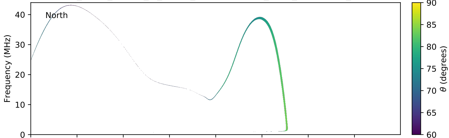
expres_earth_jupiter_io_jrm09_lossc-wid1deg_3kev_20150927_v01.cdf
