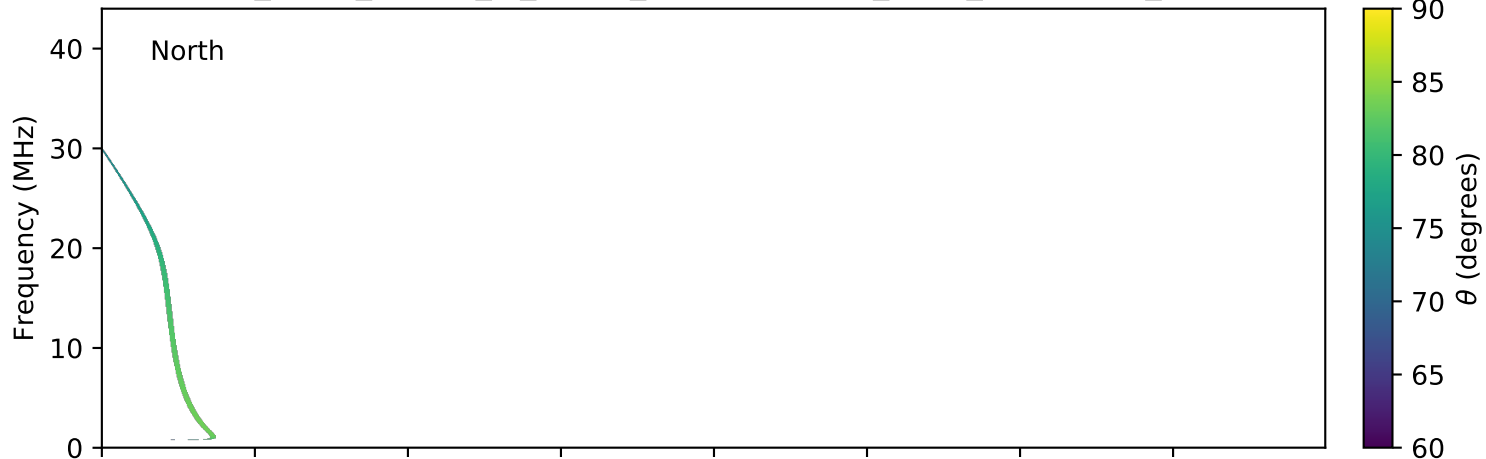
expres_earth_jupiter_io_jrm09_lossc-wid1deg_3kev_20150924_v01.cdf
