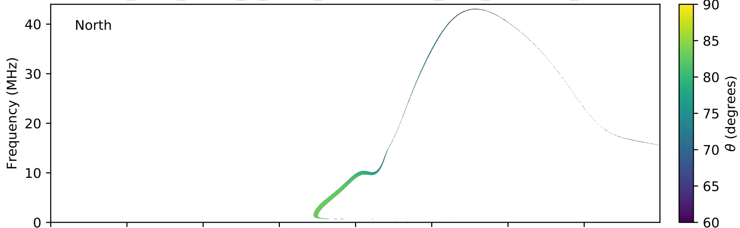
expres_earth_jupiter_io_jrm09_lossc-wid1deg_3kev_20150914_v01.cdf
