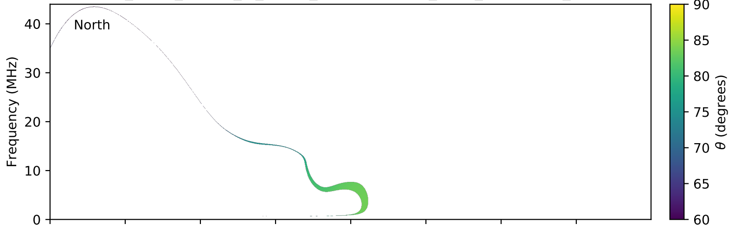
expres_earth_jupiter_io_jrm09_lossc-wid1deg_3kev_20150913_v01.cdf
