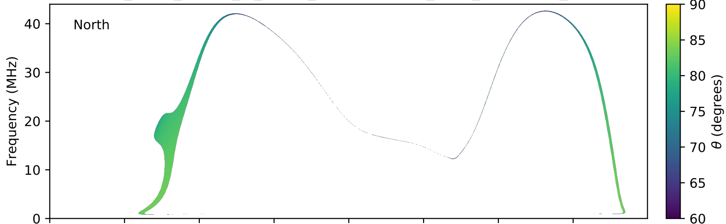
expres_earth_jupiter_io_jrm09_lossc-wid1deg_3kev_20150909_v01.cdf
