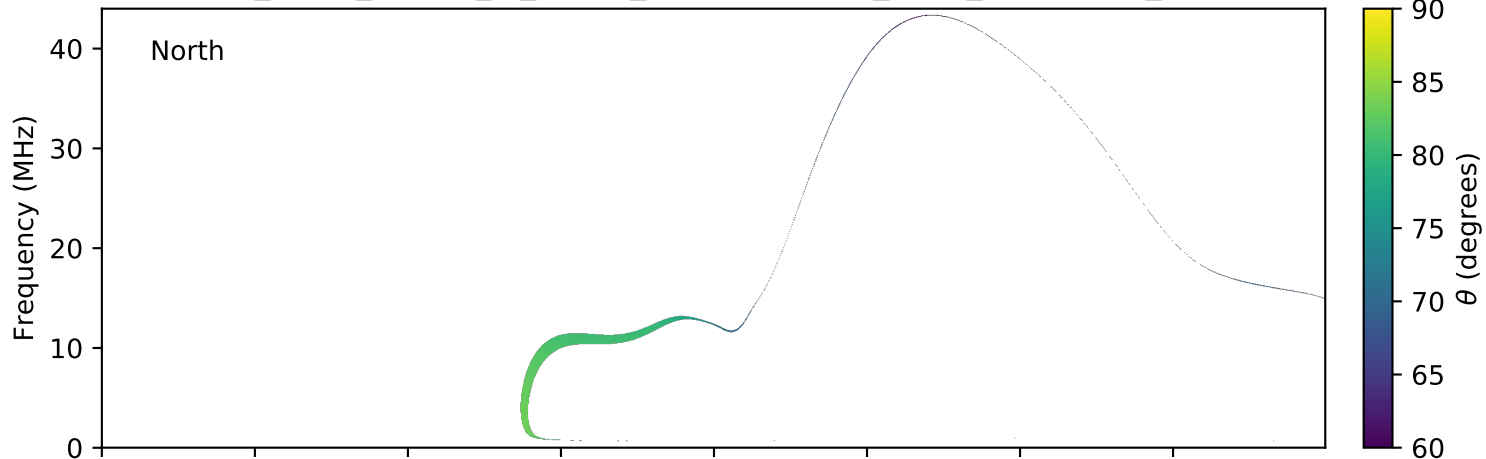
expres_earth_jupiter_io_jrm09_lossc-wid1deg_3kev_20150907_v01.cdf
