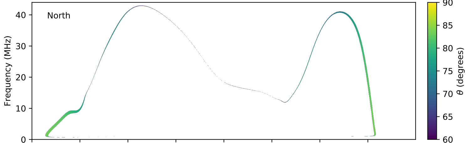
expres_earth_jupiter_io_jrm09_lossc-wid1deg_3kev_20150902_v01.cdf
