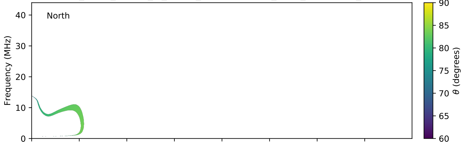
expres_earth_jupiter_io_jrm09_lossc-wid1deg_3kev_20150901_v01.cdf
