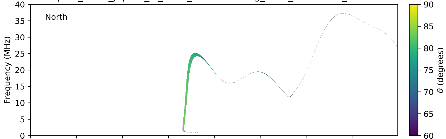
expres_earth_jupiter_io_isaac_lossc-wid1deg_3kev_20150930_v01.cdf
